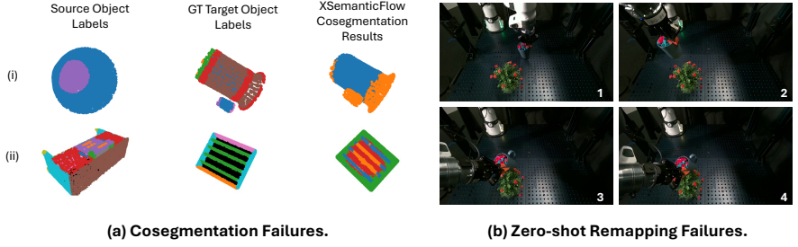
Fig. 5: Failure cases of XSemanticFlow. (a) Cosegmentation tends to fail on objects with mismatching label sets. (b) Trajectory remapping failure where the robot fails to perform the planned pouring action due to joint limit.
